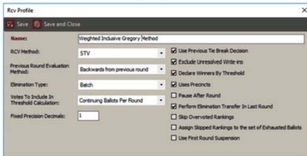
Figure 11-3: RCV Profile screen
